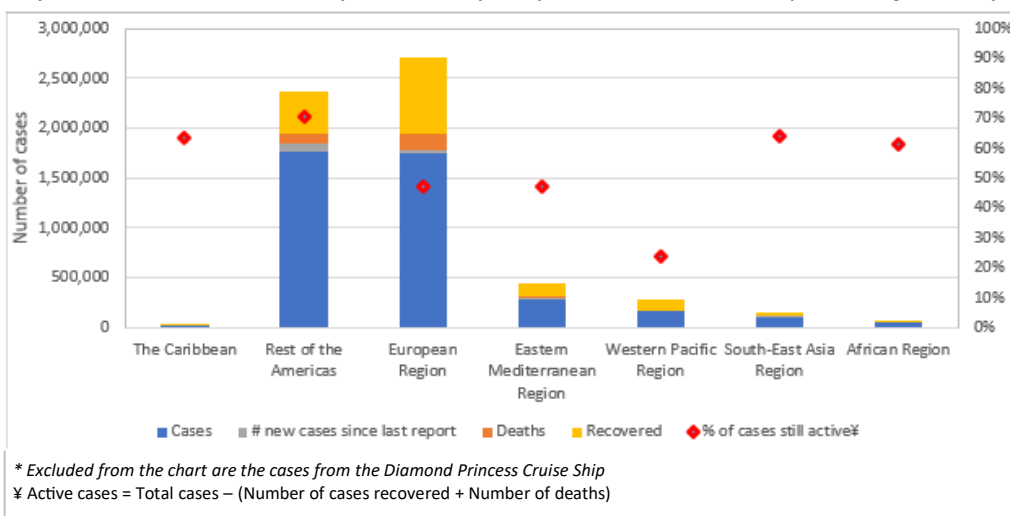
Figure 1: Reported Cases of COVID-19 by Region as of 13 May, 2020*
