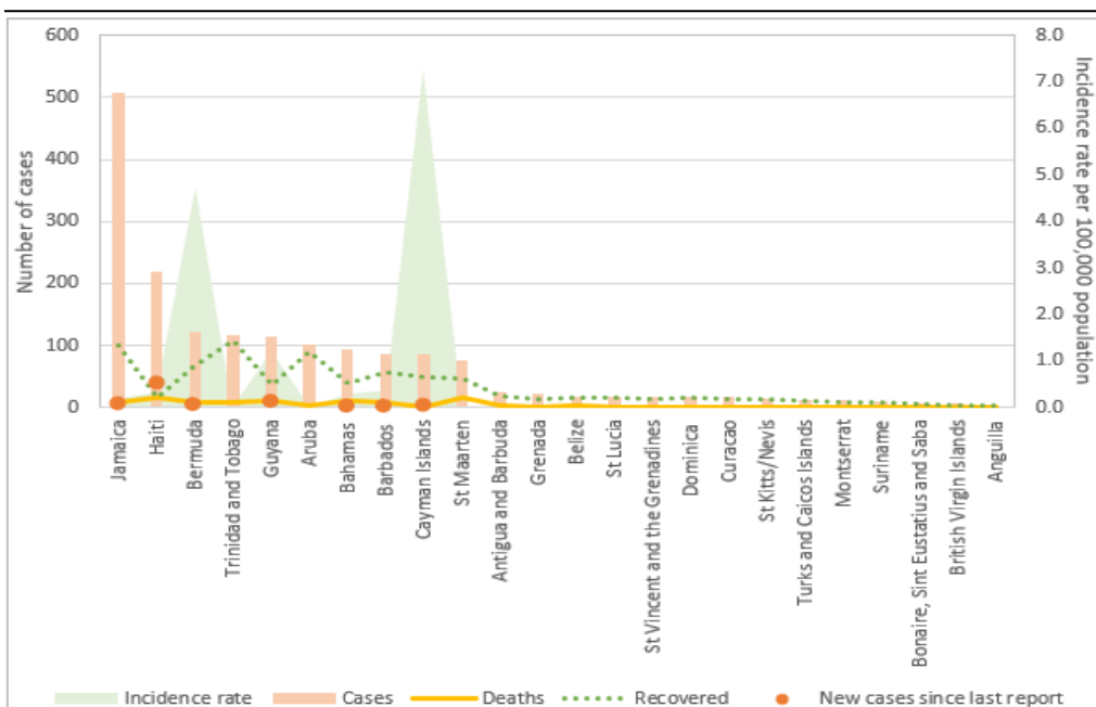
Figure 2. Confirmed Cases in Member States as of May 13, 2020
