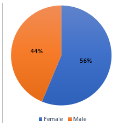
Figure 4. Percentage of Confirmed Cases of COVID-19 by sex in CMS, n=764
