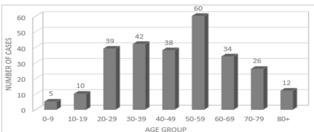
Figure 3. Reported confirmed cases of COVID-19 by age group in CMS, n=266
